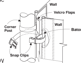
BATON WALL
